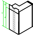
PP16 a. Exposure 16" b. Overlap 2" c. Total Length 18"
