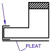
PP4 a. Exposure 4" b. Overlap 4"
