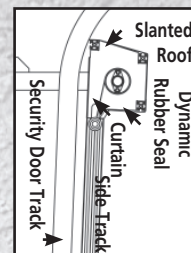
Projection Mount
