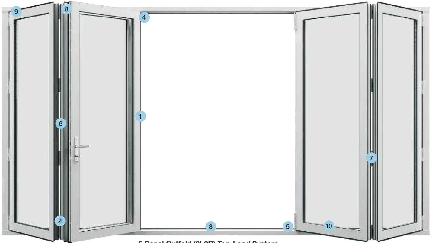
5 Panel Outfold (3L2R) Top-Load System Shown from the exterior side of the door system.
